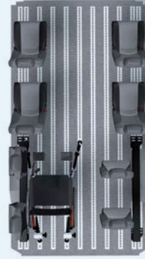
4 seats, 2 folding seats and 1 wheelchair
