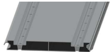
Profile Smartfloor double basic 173 (251)
