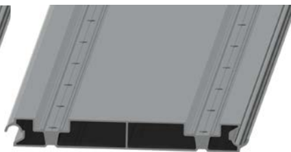
Profile Smartfloor double basic 156 (234)
