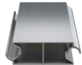
Profile Smartfloor spacer 78
